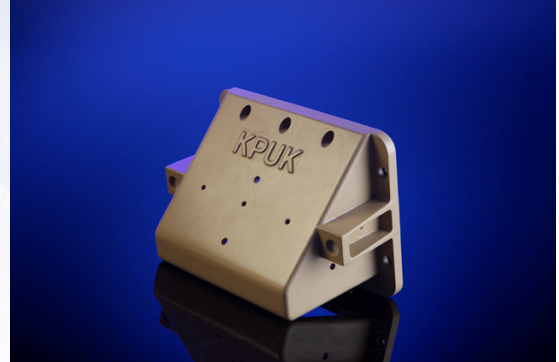
Fully finished and painted Aluminium Casting
